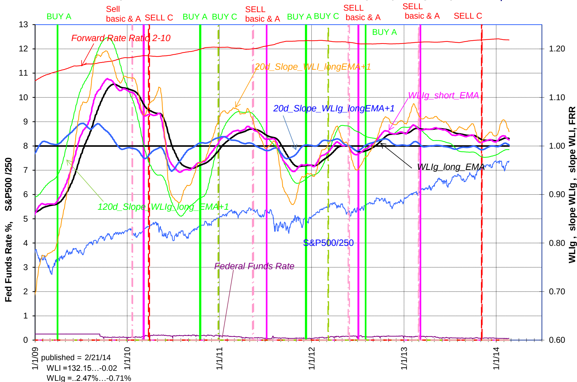
Figure 1 : 2009-13 Fed Funds Rate, S&P 500, FRR, WLlg, slope WLlg, slope WLI updated to....2/21/14
